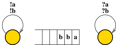
Figure 10: The infinite buffer model
