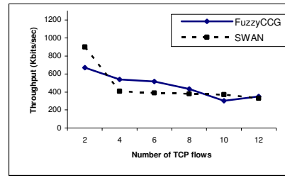
Fig. 13: Average throughput in FuzzyCCG and SWAN models vs. number of TCP flows
