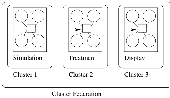
Figure 1. Application Model
