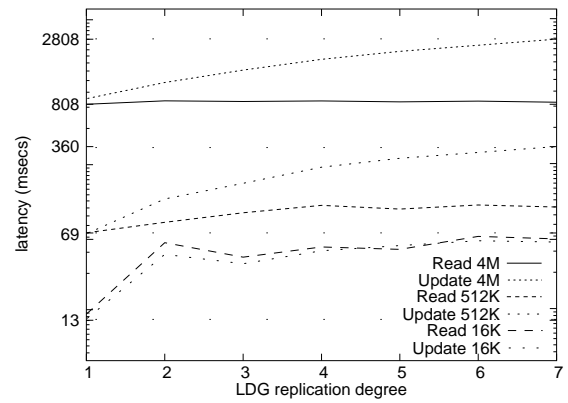
Figure 6. Cost of the basic primitives: read/update.
