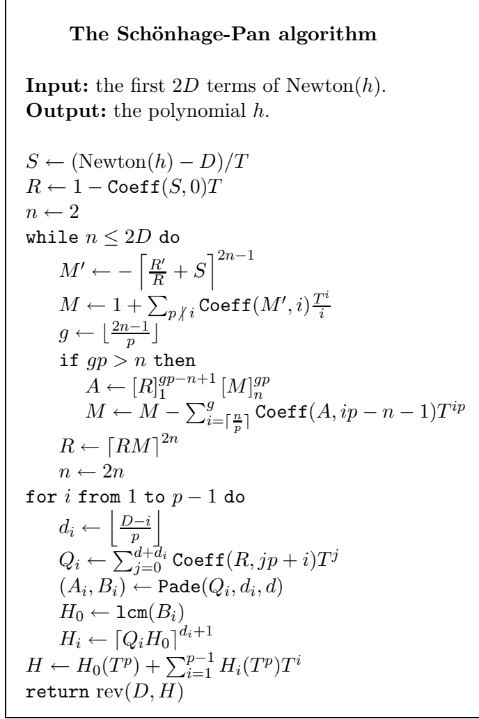
Fig. 3. Recovering a monic polynomial from its Newton series in small characteristic
