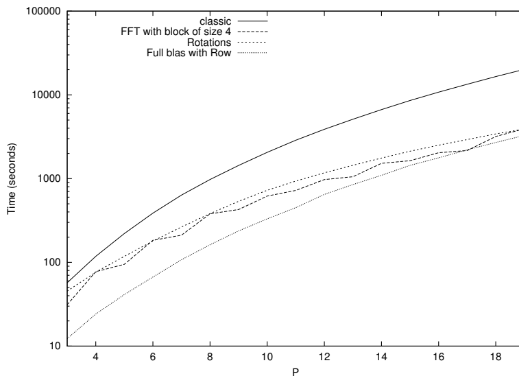
Figure 13: Logarithmic downward pass CPU times of the different M2L computation schemes, for an octree of height 5 and with double height M2L kernel. Tests are performed on an IBM Power3 with 2 GB of memory.
