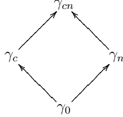
Figure 7. \gamma -calculi.
