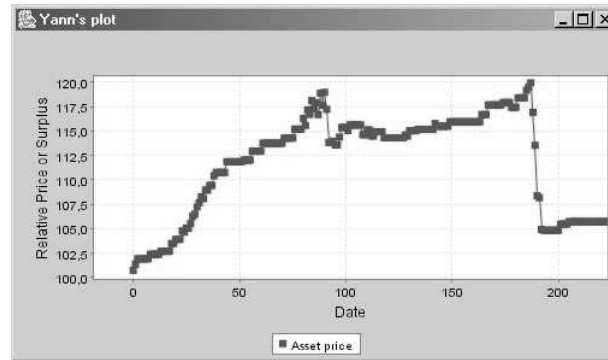
Fig. 6. A speculative bubble obtained with R_0 in U_{[0.4;0.8]} , w = -5 and asymmetric pricing when agents are panicking
