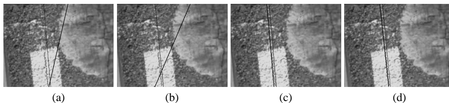
Fig. 4. Fitting on a real image assuming (a) Gauss, (b) quasi-Laplace, (c) Cauchy, and (d) Geman & McClure distributed noise. Thin black lines are the initial A_0 's. Thick ones are the fitting results. See Sec. 4 for a definition of the pdfs.
