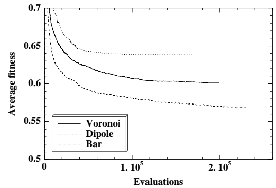
Average fitness values averaged over 21 runs
