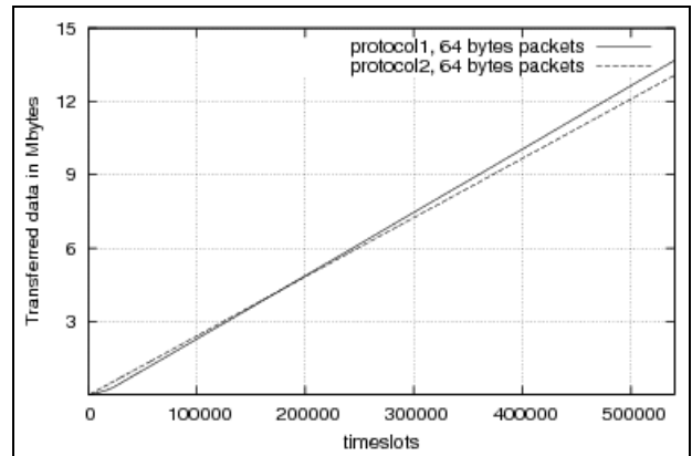
Figure 8 Transferred payload data in random 100 network.
