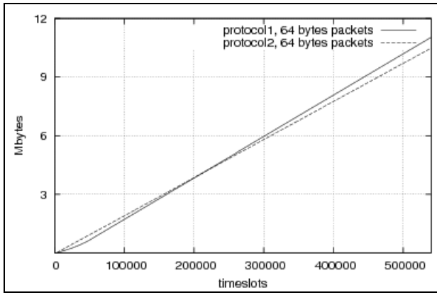
Figure 9 Transferred payload data in random 200 network.
