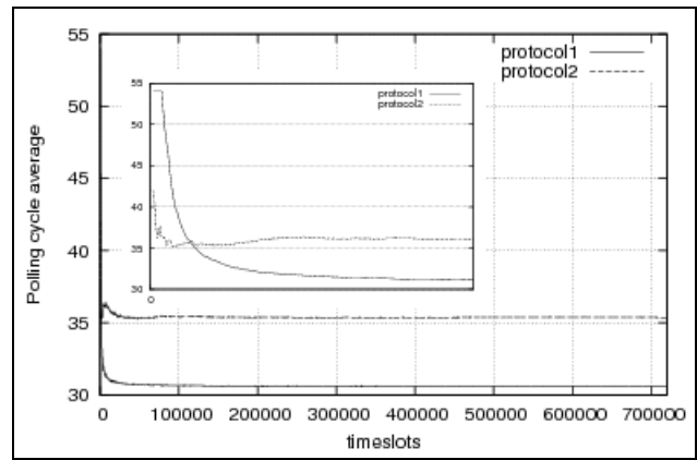
Figure 2 Polling cycle average for ring 10 network with start-up phase zoom.
