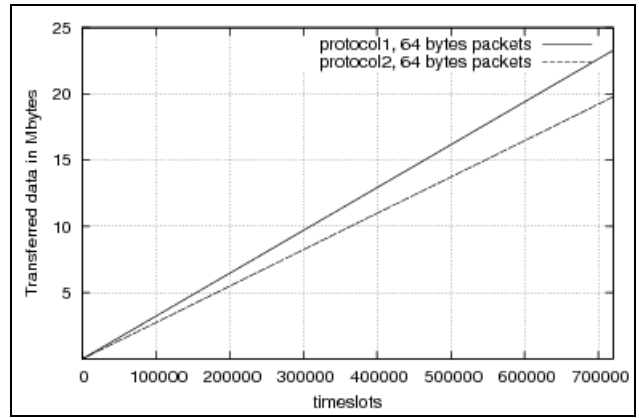
Figure 6 Transferred payload in ring 10 network.
