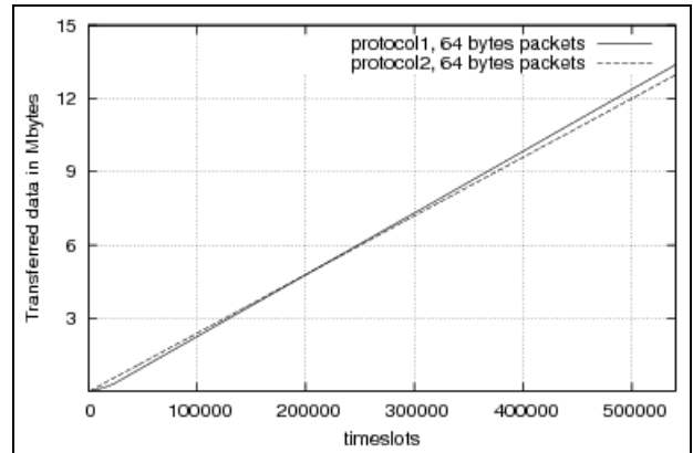
Figure 7 Transferred payload data in ring 100 network.
