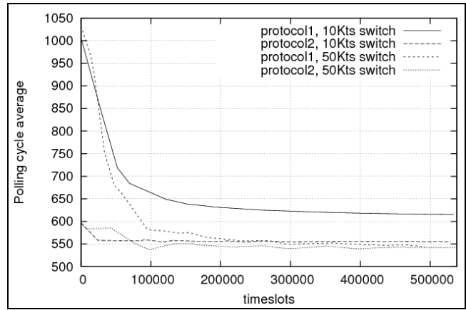
Figure 10 Polling cycle average comparison for open ring 100 network.
