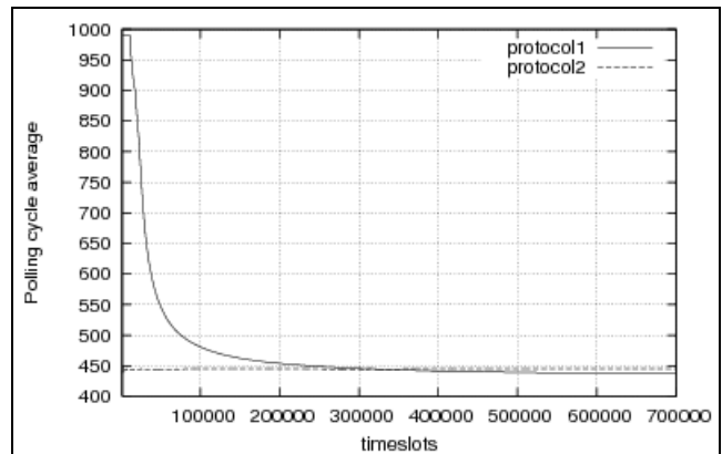
Figure 3 Polling cycle average for ring 100 network.
