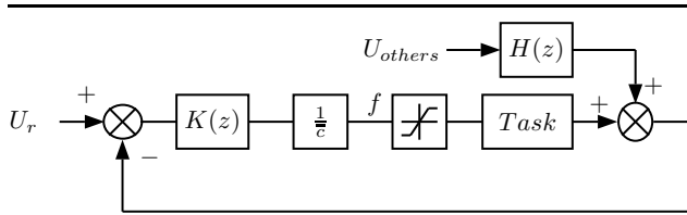
Figure 3. Control scheme for CPU resources
