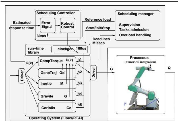
Figure 8. Feed-back scheduling experiment
