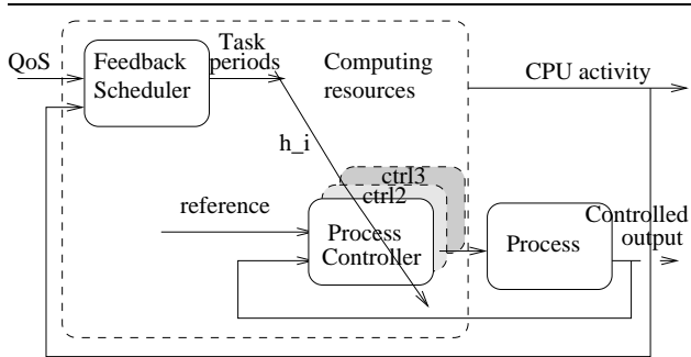
Figure 1. Hierarchical control structure
