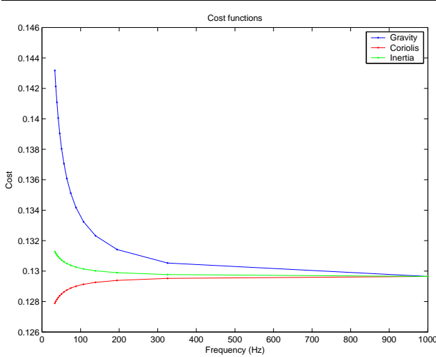
Figure 4. Cost functions
