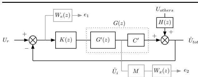
Figure 5. H_\infty design bloc diagram
