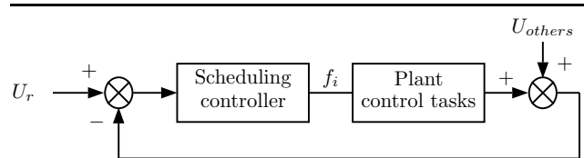
Figure 2. Feedback scheduling bloc diagram
