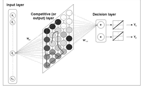
Figure 1: From left to right, the first two layers represent the general architecture of the Self Organizing Map (SOM): X_i(i=1...23) input corresponds to the percentage of the power spectrum of I band (PSSi). W_{p,n}(p=1...23, n=1...25) weights from input to competitive layer. The other two layers indicate the principle of Learning Vector Quantization (LVQ)
