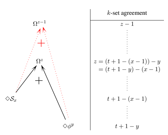
Figure 2: Additivity of \Diamond S_x and \Diamond \phi^y
