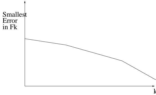
Fig. 1. Illustration of the proof. With a larger k , \mathcal{F}_k has a smaller best error.
