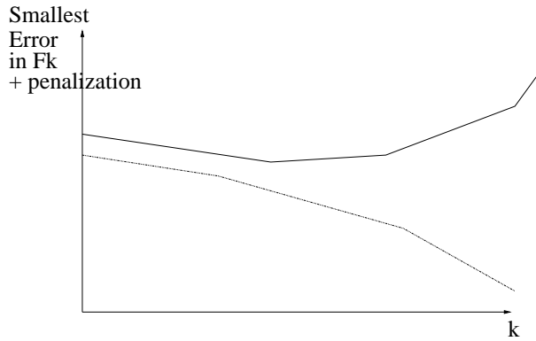
Fig. 2. Illustration of the proof. With a larger k , \mathcal{F}_k has a smaller best error, but the penalization is stronger than the difference of error.
