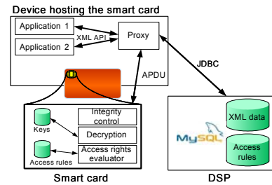
Figure 3. Architecture
