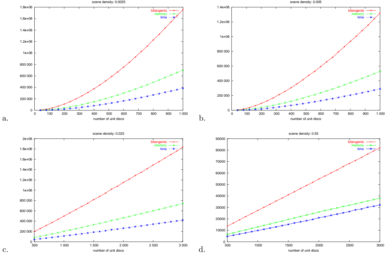
Figure 2: Plots of the number of directed bitangents, memory usage, and running time versus the number of unit discs, when scene density is a. \mu = 0.0025 , b. \mu = 0.005 , c. \mu = 0.025 , d. \mu = 0.55 . The unit of the memory usage is kB, that of the running time is 10^{-4} seconds.
