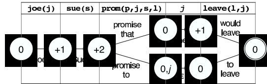
Figure 1.5: Constructing a polarity automaton with zero-literal semantics.
