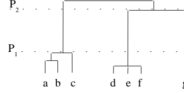
Fig. 2. Hierarchy partitioning
