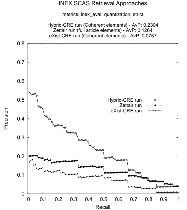
Figure 3: Evaluation of the XML retrieval approaches by using strict quantisation function in inex_eval .
