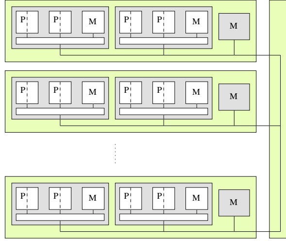
(a) A NUMA of HyperThreaded multicores.
