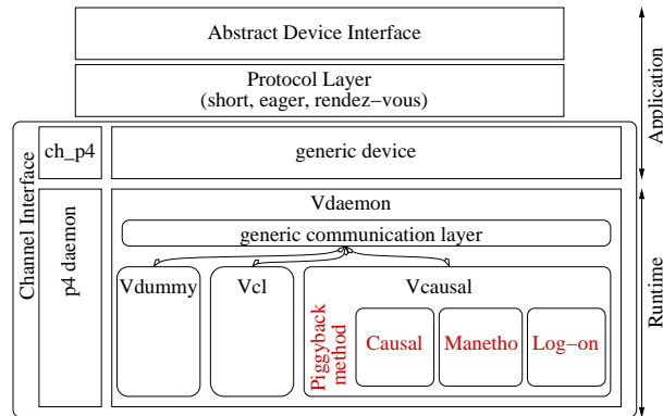
Fig. 4. General Architecture of MPICH-V compared to the architecture of MPICH-P4
