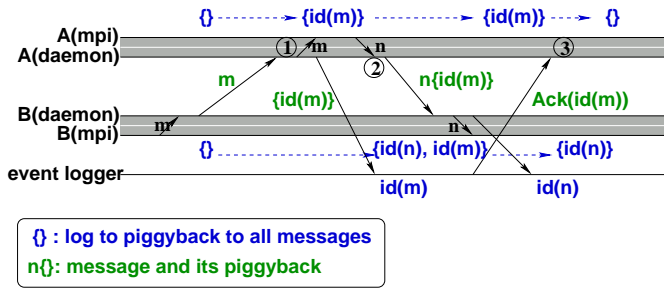
Fig. 2. Sample of execution without fault of a causal logging protocol with an Event Logger
