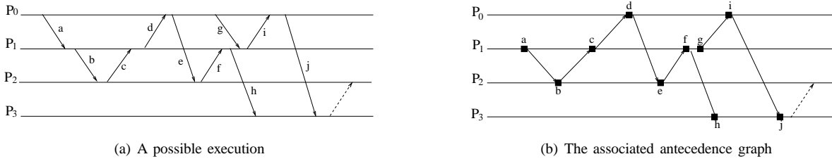
Fig. 3. Example of causal protocol execution and the resulting antecedence graph
