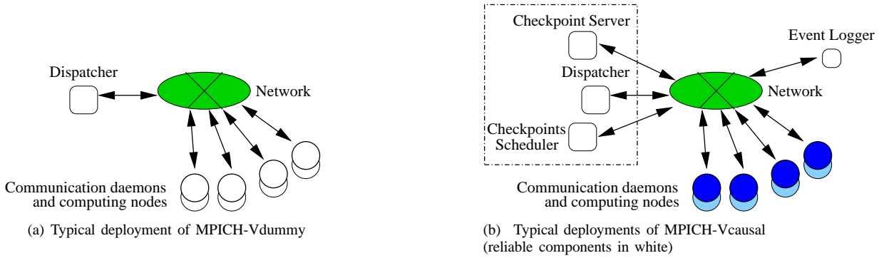
Fig. 5. Components of the MPICH-V framework
