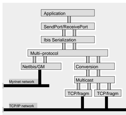
Figure 2. The NETIBIS architecture.
