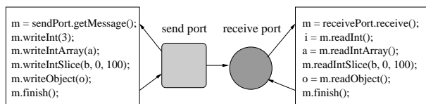
Figure 1. The IPL communication abstraction.
