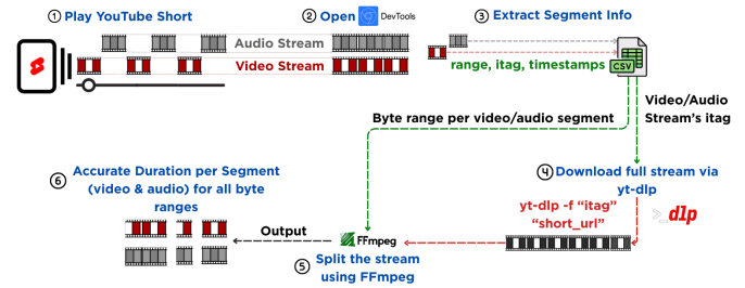
Figure 1: Pipeline to derive accurate segment durations using DevTools, yt-dlp, and FFmpeg.
