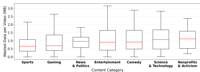
Figure 4: Distribution of wasted data per video for Scenario 3 (skip at 10 s). Boxes show interquartile range, whiskers show full range, and the red line marks the median.
