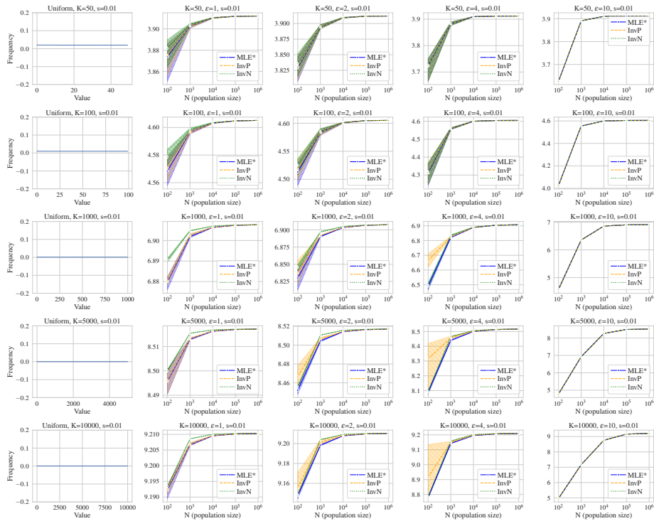
Figure 8: Negative log-likelihood results for near-uniform distribution ( s = 0.01 ). Rows vary domain size K , and columns vary privacy level \epsilon . The far-left subplot of each row shows the true histogram.
