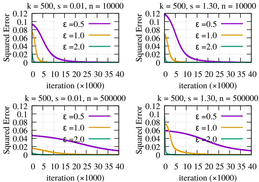
Figure 4: The squared error of the IBU's estimates relative to MLE*, with the number of iterations.
