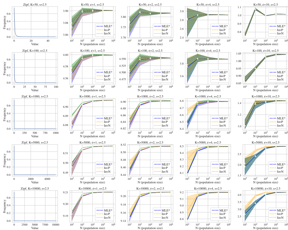
Figure 10: Negative log-likelihood results for highly concentrated distribution ( s = 2.5 ). Rows vary domain size K , and columns vary privacy level \epsilon . The far-left subplot of each row shows the true histogram.
