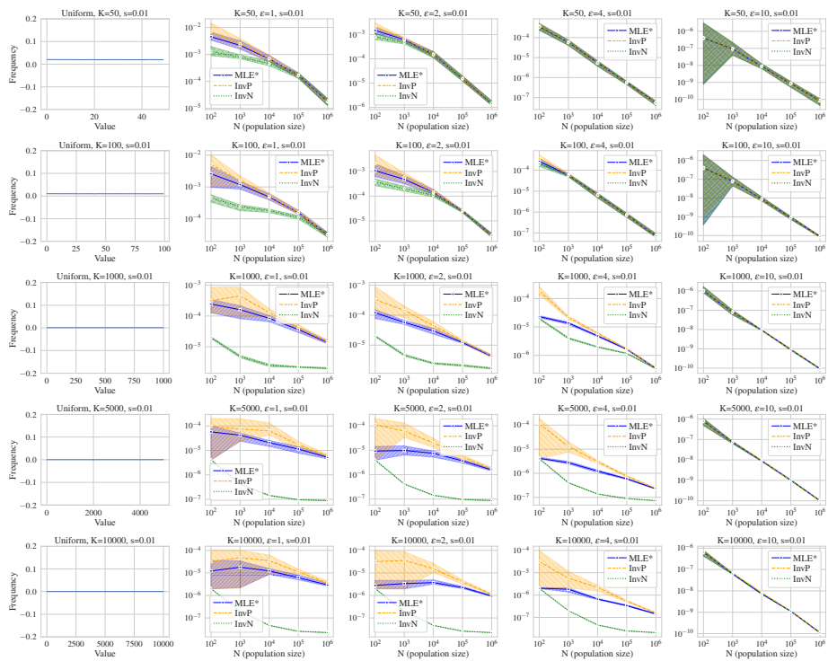
Figure 5: MSE results for near-uniform distribution ( s = 0.01 ). Rows vary domain size K , and columns vary privacy level \epsilon . The far-left subplot of each row shows the true histogram.
