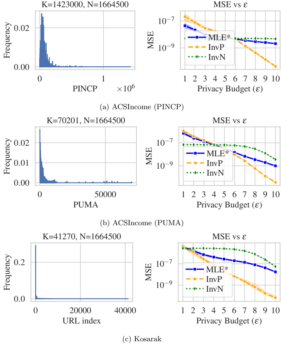
Figure 3: Performance of MLE*, InvP, and InvN across three different real-world distributions.
