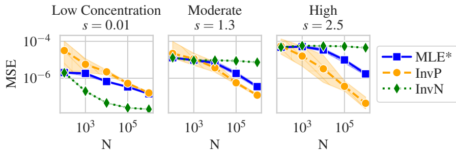
(a) Mean Squared Error (MSE), K = 10000, \epsilon = 4
