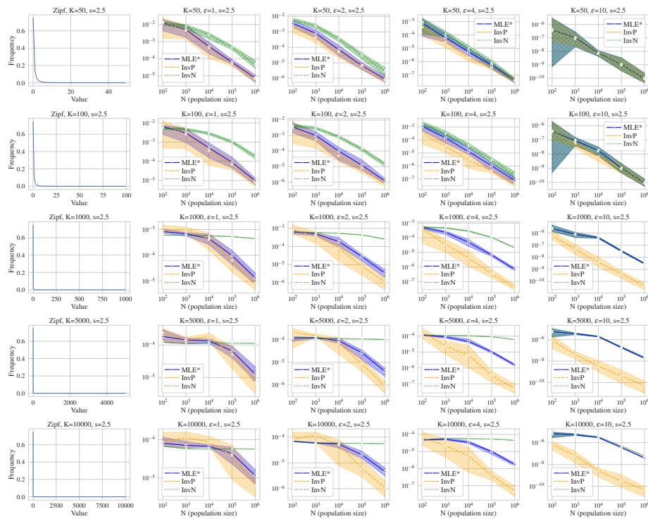
Figure 7: MSE results for highly concentrated distribution ( s = 2.5 ). Rows vary domain size K , and columns vary privacy level \epsilon . The far-left subplot of each row shows the true histogram.
