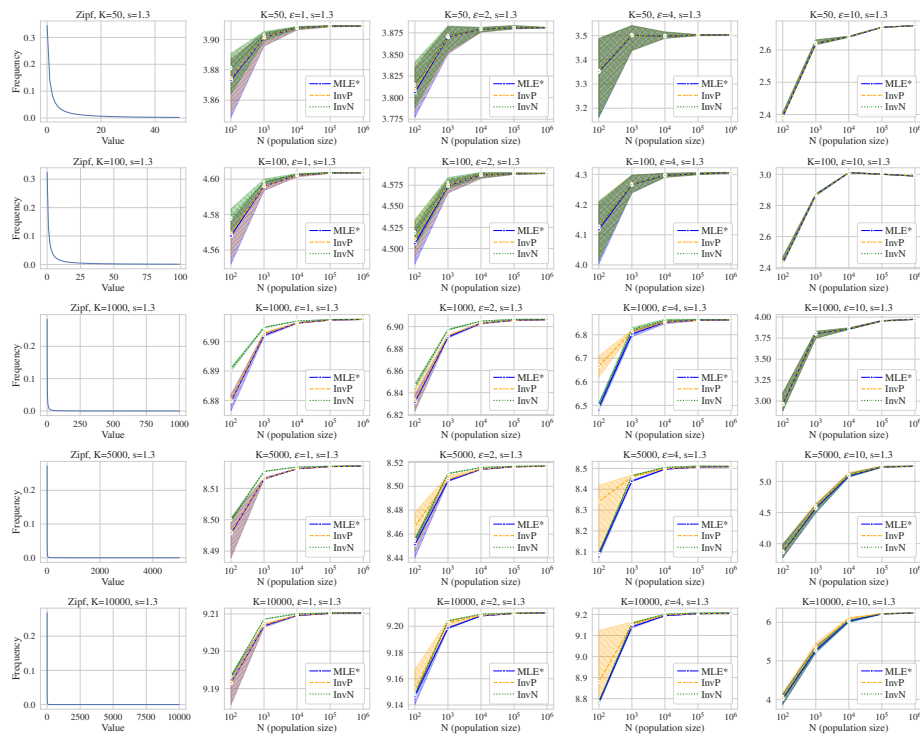
Figure 9: Negative log-likelihood results for moderately skewed distribution ( s = 1.3 ). Rows vary domain size K , and columns vary privacy level \epsilon . The far-left subplot of each row shows the true histogram.
