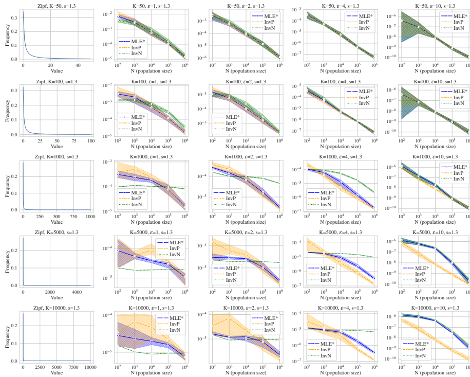
Figure 6: MSE results for moderately skewed distribution ( s = 1.3 ). Rows vary domain size K , and columns vary privacy level \epsilon . The far-left subplot of each row shows the true histogram.
