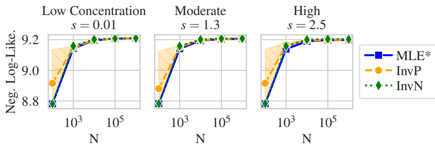
(b) Negative Log-Likelihood, K = 10000, \epsilon = 4
