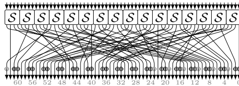
(a) GIFT-64 round function.
