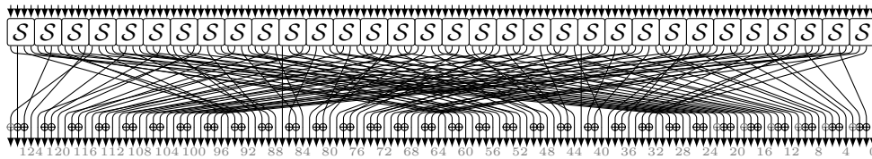
(b) GIFT-128 round function.
