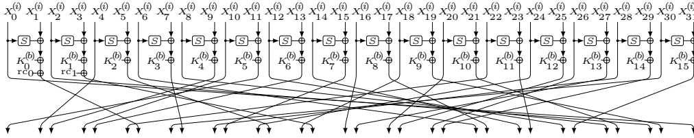
Figure 10: The round function of WARP, where the round key index is b = i \bmod 2 .
