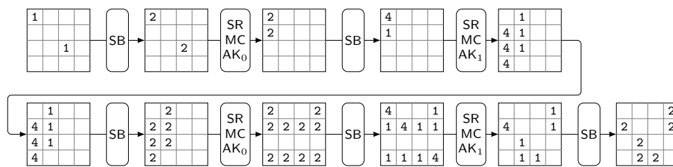
(a) Differential characteristic, first to last S-box layer.
