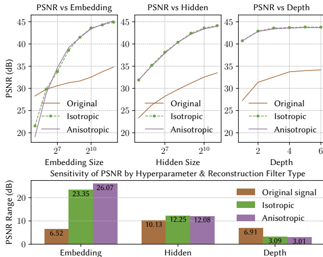
Fig. 4. Sensitivity Analysis. We evaluate how Fourier-feature embedding size and network architecture affect (1) reconstruction of the original signal, (2) isotropic smoothing, and (3) anisotropic smoothing. Embedding Size. While embedding size has relatively smaller effect on reconstructing the original signal, the model benefits substantially from larger embeddings in both isotropic and anisotropic smoothing tasks. Hidden Dimension. Increasing the hidden-layer width consistently yields higher PSNR across all tests. Network Depth. Adding more than three layers provides only marginal PSNR gains, indicating diminishing returns beyond a depth of three. The bottom row shows the PSNR range (highest minus lowest) observed over each hyperparameter sweep, illustrating the relative sensitivities.
