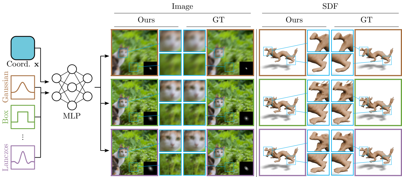
Fig. 1. We present a training method for neural fields that enables linear prefiltering with multiple reconstruction filters. At training time, the neural field sees parameters of a single symmetric filter. At test time, we support prefiltering a variety of unseen filters (e.g., Box or Lanczos). Here, we show neural fields trained on an image (with bottom-right insets of frequency spectrum) and signed distance function using Gaussian filters, with generalization on Box and Lanczos filters. Images from Adobe FiveK; © original photographers/Adobe. Mesh models from the Stanford 3D Scanning Repository; © Stanford Computer Graphics Laboratory. (Project page: https://myaldiz.info/assets/spnf/ )
