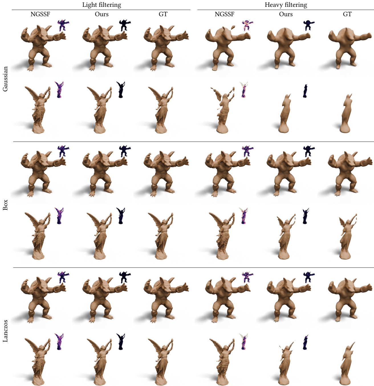
Fig. 7. Filter generalization on SDFs. Comparisons against recalibrated Neural Gaussian Scale-Space Fields [Mujkanovic et al. 2024] (NGSSF) for SDF filtering with different kernels. Insets at the top-right represent the distance to the ground truth mesh, darker is better. Our model shows closer geometry to the ground-truth compared to NGSSF. Mesh models from the Stanford 3D Scanning Repository; © Stanford Computer Graphics Laboratory.
