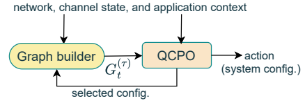
Fig. 3. QIC solution framework.
