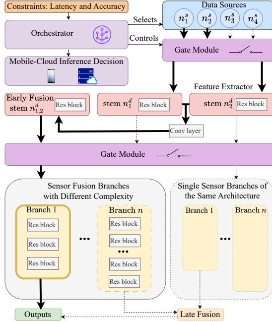
Fig. 2. Architecture implemented for object detection inference, illustrating the process where the orchestrator selects the data source, followed by the gate modules determining the appropriate stem and branch for deployment.
