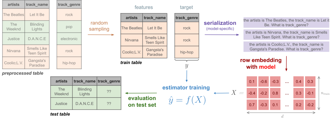
Figure 4: An overview of our evaluation pipeline. For each dataset, we sample training and test sets. We then serialize the rows and use the embedding model to generate a vector representation for each row. Finally, we train a tabular learning estimator to evaluate these embeddings.
