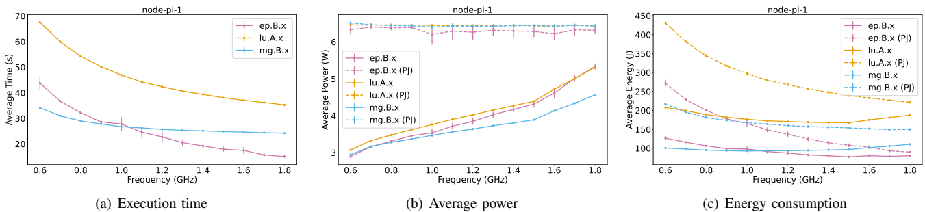
Fig. 2. Experiments run on one IoT edge node with different CPU frequency for the three NAS parallel benchmarks. Power is measured by external monitoring and estimated by PowerJoular. Each point is an average over 10 runs. The standard deviation is also reported.
