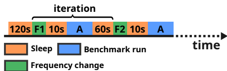
(a) Experiment phases for the NAS parallel benchmarks.
