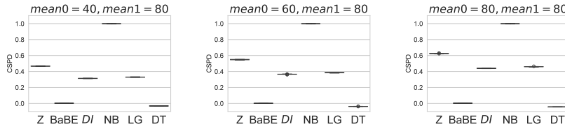
Fig. 8. Experiments on the synthetic data sets: Conditional Statistical Parity Difference (CSPD). We recall that, for BaBE, DI, NB, LG and DT, the CSPD is defined as \mathbb{P}[\hat{Y}_{\hat{E}} = 1|E, S = 1] - \mathbb{P}[\hat{Y}_{\hat{E}} = 1|E, S = 0] . For Z , the definition is similar, with \hat{Y}_{\hat{E}} replaced by Y_Z .
