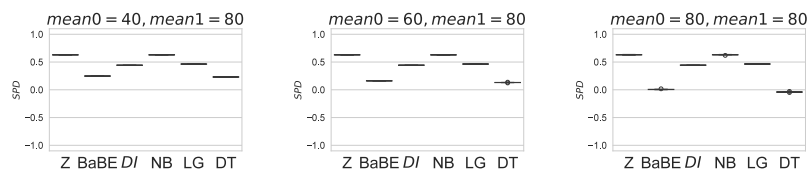
Fig. 10. Experiments on the synthetic data sets: Statistical Parity Difference (SPD). We recall that, for BaBE, DI, NB, LG and DT, the SPD is defined as \mathbb{P}[\hat{Y}_E = 1 | S = 1] - \mathbb{P}[\hat{Y}_E = 1 | S = 0] . For Z, the definition is similar, with \hat{Y}_E replaced by Y_Z .
