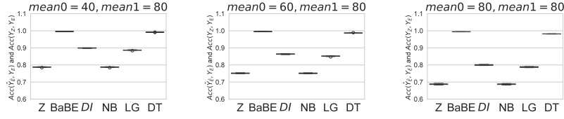
Fig. 6. Experiments on the synthetic data sets: The accuracy between \hat{Y}_Z and Y_E , and between \hat{Y}_{\hat{E}} and Y_E .
