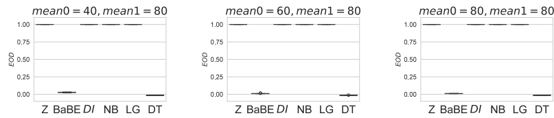
Fig. 9. Experiments on the synthetic data sets: Equal Opportunity Difference (EOD). We recall that, for BaBE, DI, NB, LG and DT, the EOD is defined as \mathbb{P}[\hat{Y}_E = 1 | Y_E = 1, S = 1] - \mathbb{P}[\hat{Y}_E = 1 | Y_E = 1, S = 0] . For Z, the definition is similar, with \hat{Y}_E replaced by Y_Z .
