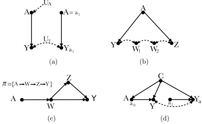
Figure 8: Causal graphs.
