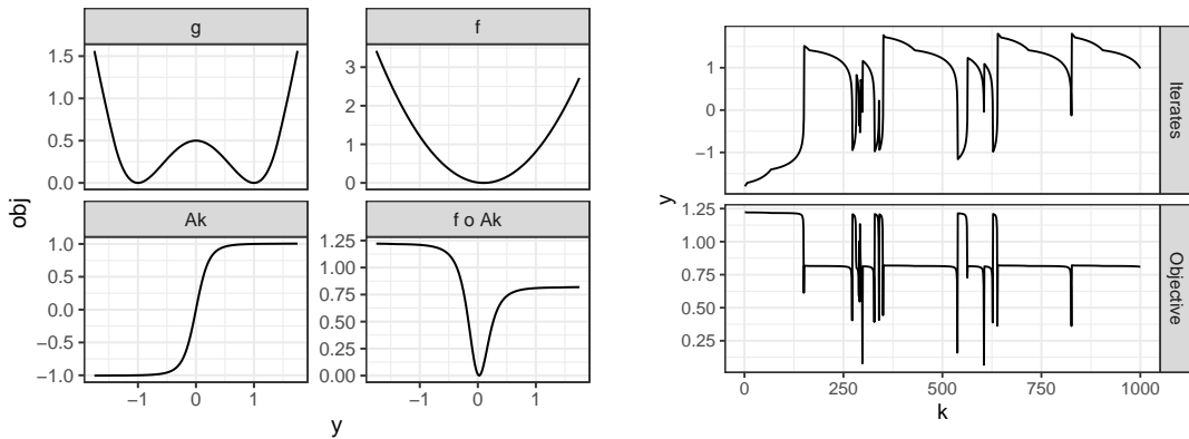
Figure 2: Illustration of the instability phenomenon of the diagonal method. Left: inner objective g and outer objective f , with the outcome of k gradient steps on g , depending on the initialization \mathcal{A}^k(z) and the corresponding approximation \varphi^k(z) = f(\mathcal{A}^k(z)) . Right: value of \varphi^k along iterations. Many iterations have objective values corresponding to solutions of the bilevel problem (BL) but tends to be attracted by the sharp global minimizer of f , which is repulsive for Algorithm DPBG.
