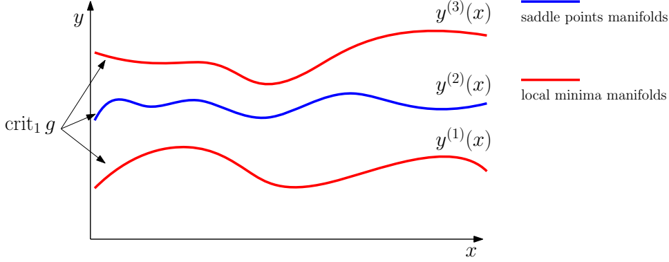
Figure 1: Structures of \text{crit}_1 g (see definition in Section 2.1) under Assumption Morse QC see Proposition 3.6. The decomposition of the set of critical points and local minima of g as a finite union of manifolds are represented by several functions y^{(1)}(x), y^{(2)}(x), y^{(3)}(x) . The saddle point manifolds (in blue) and local minima manifolds (in red) illustrate the stratification of the critical set.
