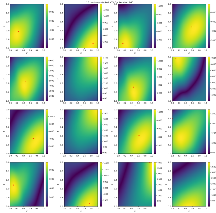
Figure 11: NTK at the end of optimization for Laplace equation in 2 D. Reading: the red cross on each subfigure representing a point x_i , the plot represents the function NTK_{\theta_{\text{end}}}(\cdot, x_i)
