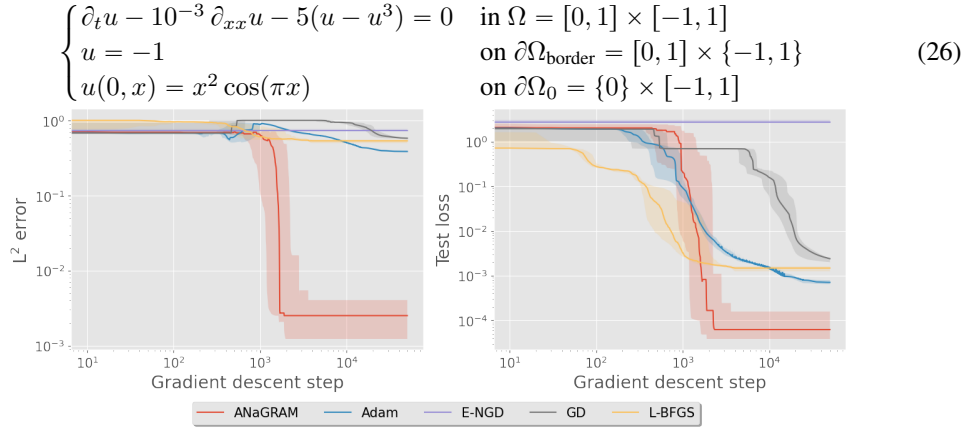
Figure 4: Median absolute L^2 errors and Test losses for the Allen-Cahn equation.
