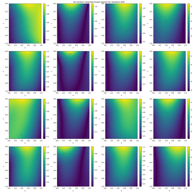
Figure 20: Green’s function of the operator on the tangent space at the end of optimization for Heat equation in 1+1 D. Reading: the red cross on each subfigure representing a point x_i , the plot represents the function g_{T_{\theta_{\text{end}}}\mathcal{M}}(\cdot, x_i)
