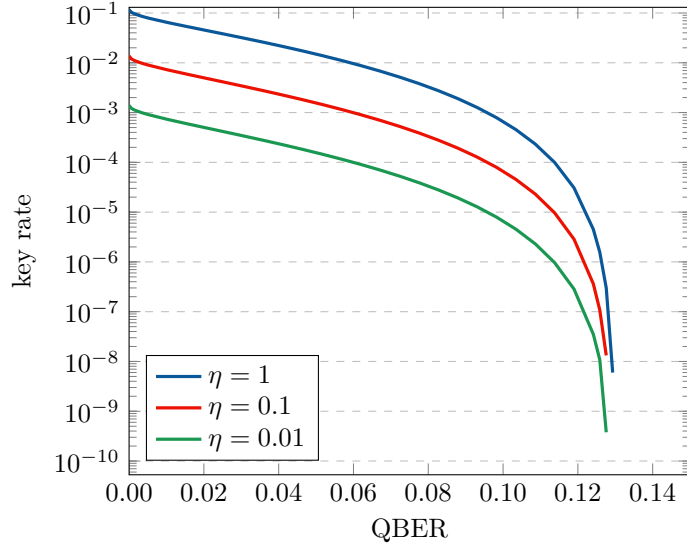
Figure 9: Asymptotic key rate in the limit n \rightarrow \infty for different QBERs and transmittances. We choose \alpha to optimize the key rates. Note that a secret key can be distilled up to a threshold QBER \approx 13\% independent of transmittance.
