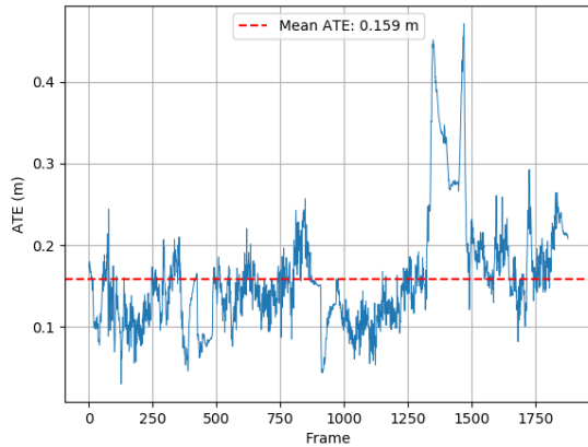
Figure 10. Our method exhibits consistent ATE behavior over 1900 frames, showing stability at various distances across multiple experiments. However, a notable shift occurs when the model is observed in regions with extremely low-texture conditions.
