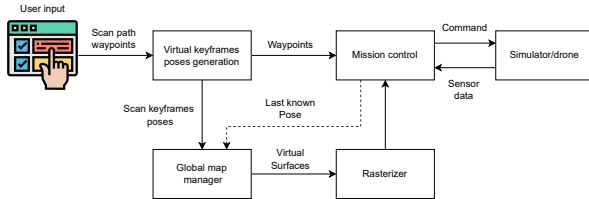
Figure 5. The global map manager will take any pose and generate a virtual surface that will be used to generate a depth and color images necessary for the odometry.
