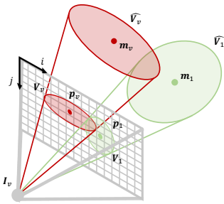
Figure 2. The 3D covariance matrices in camera frame \hat{V}_1, \dots, \hat{V}_v are mapped as ellipsoid regions in the image space \mathbf{V}_1, \dots, \mathbf{V}_v through perspective projection linearized around the center of the ellipsoids \mathbf{m}_1, \dots, \mathbf{m}_v whose coordinates in the image plane are \mathbf{p}_1, \dots, \mathbf{p}_v . Then the colors are merged by means of a weighted average.
