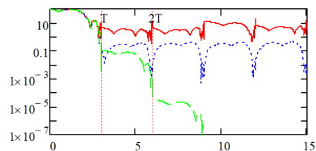
Figure 2. The state norm versus time t , h = 0.01
