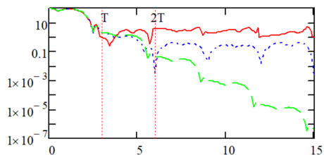
Figure 1. The state norm versus time t , h = 0.1
