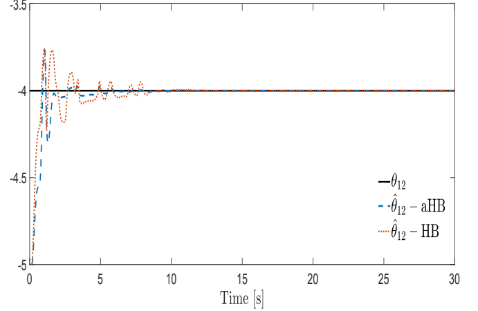
Figure 2. Parameter Identification \theta_{12}
