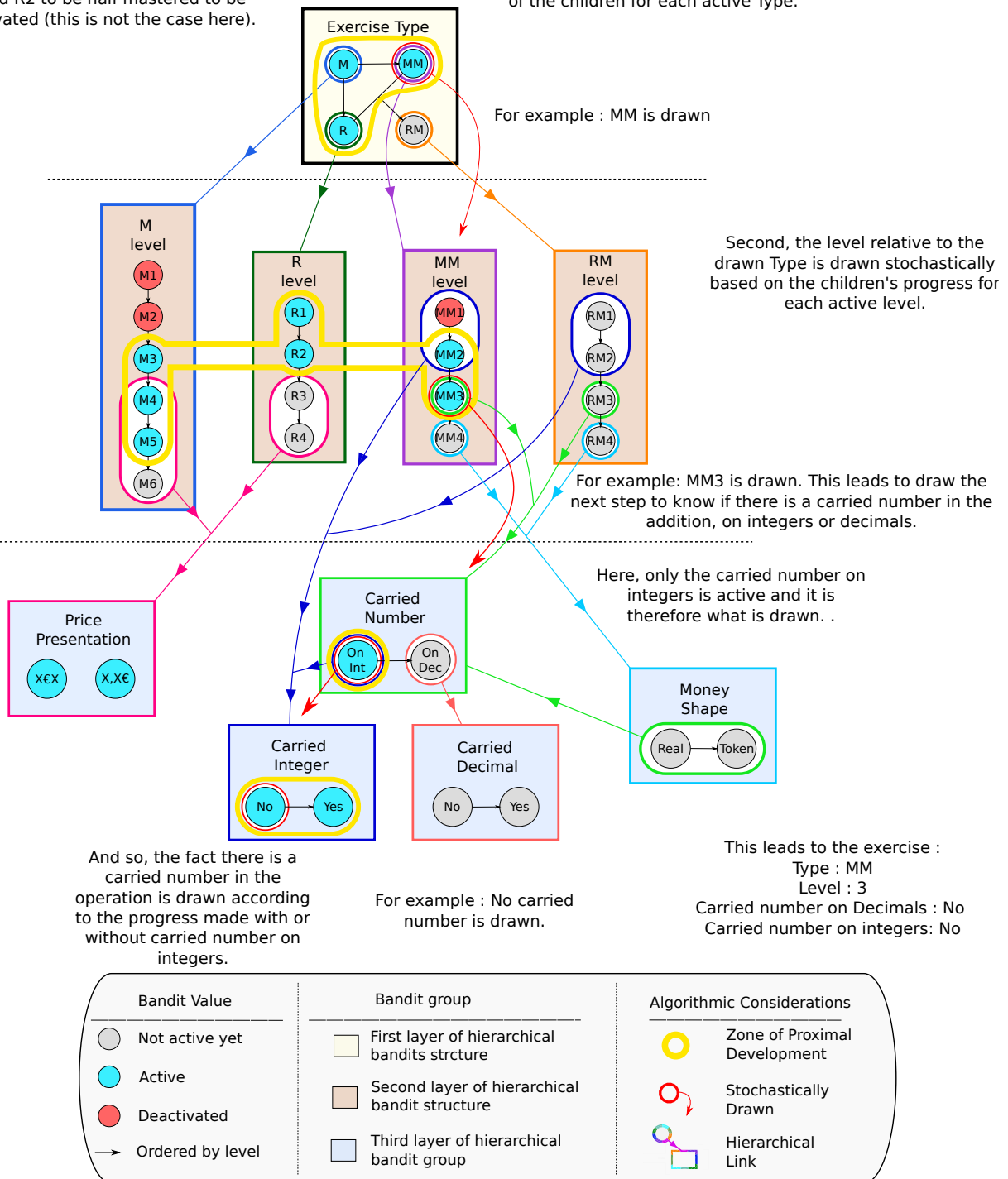
Figure 13: A representation of the activity graph used for a pedagogical scenario to teach child about mathematics by making them manipulate money. An example of activity is sampled at a particular state of the algorithm resulting from activities already made by a hypothetical student.
