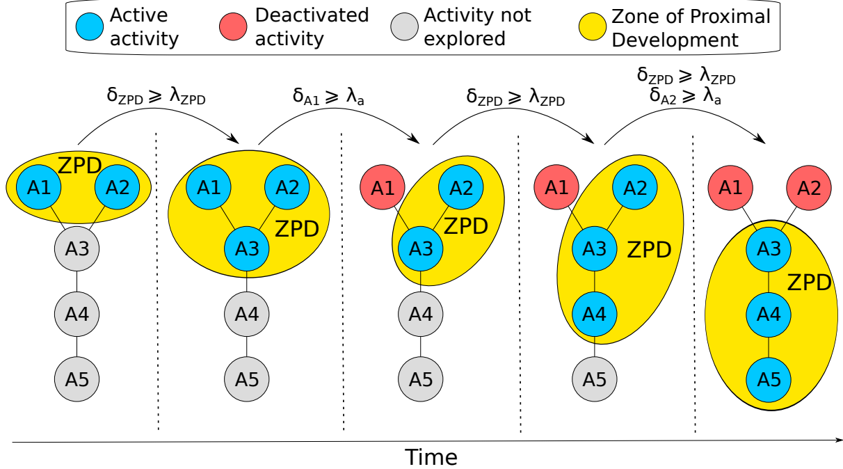
Figure 10: ZPDES exploration of an activity space, with \delta_{ZPD} the success rate over all active activities, \lambda_{ZPD} the threshold to expand the ZPD, \delta_{Ax} the success rate for the activity Ax , and \lambda_a the threshold to reach to deactivate an activity.
