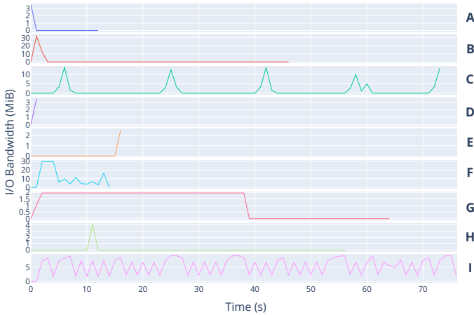
Fig. 8: An example job of each identified category. The x axis shows time, the y axis the bandwidth, and the letters identify the categories. All remaining jobs that do not fit in a category are contained in a heterogeneous set, not represented.
