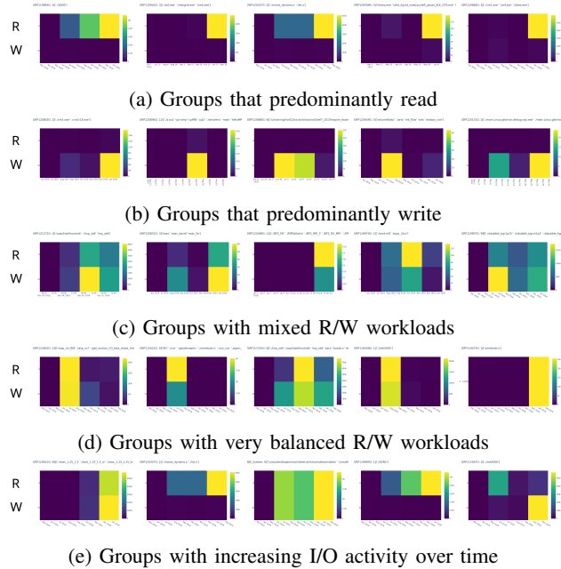
Fig. 5: Examples of group I/O activity over time
