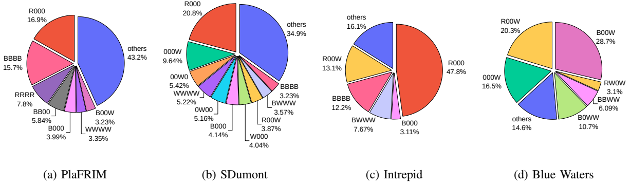
Fig. 1: Temporal I/O behavior. “Others” combine all the classes that account for less than 3% of the jobs.
