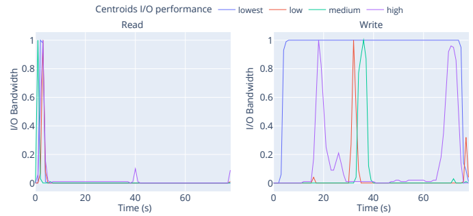
Fig. 9: Centroid of each dominant cluster per group across read and write time series of length 80. The x axis shows time, while the y axis the normalized bandwidth values of each centroid with respect to its maximum value, so that we can compare the trends between centroids.
