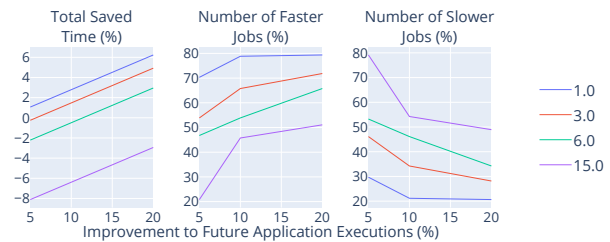
Fig. 4: Results achievable by techniques that use information from a previous run to improve performance in the next ones
