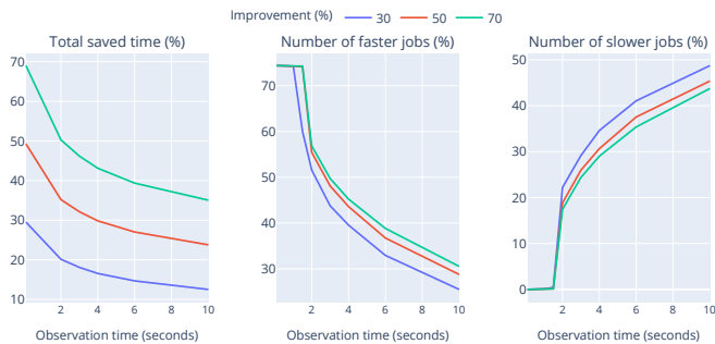
Fig. 3: Impact of techniques that improve performance after observing the job for a certain time (x axes) depending on the expected improvement on future accesses (the colors).
