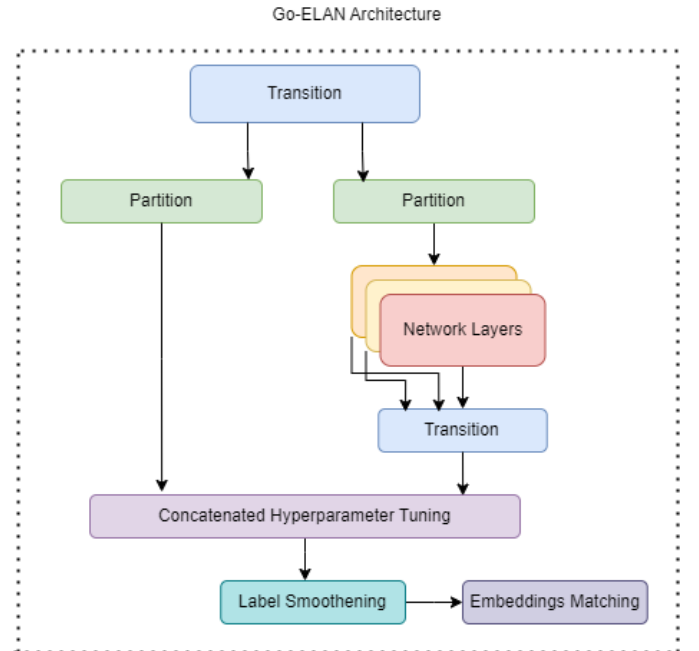
Fig. 2: Go-ELAN Architecture: Size of downsampling filters increases from 128 in GELAN to 512 in Go-ELAN to accommodate greater spatial context. A label smoother is added in the loss computer to spread out the probability mass.
