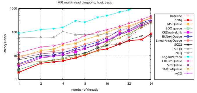
Fig. 15. Multi-threaded communication benchmark on machine pyxis
