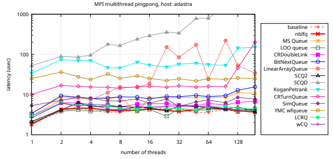
Fig. 14. Multi-threaded communication benchmark on machine adastra
