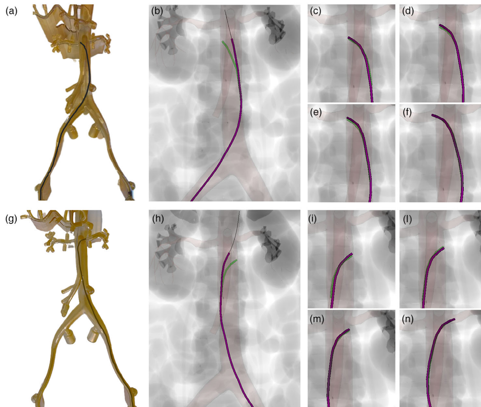
FIGURE 5 Validation study. The guidewire and the catheter equipped with the optical fibre are inserted inside a phantom in the right (top row) and left (bottom row) iliac artery. The system, besides the real instruments' shape and position ((b) and (h) in purple), shows the predicted catheter shape after guidewire withdrawal ((b) and (h) in green). (c–f, i–n) The comparison between the predicted catheter shape computed by our system (in green) and the real catheter shape obtained after guidewire withdrawal (in purple) and acquired through the optical fibre system. A mean 3D error of 2.4 \pm 1.3 mm and 2D error of 1.1 \pm 0.7 mm were measured between the two shapes.
