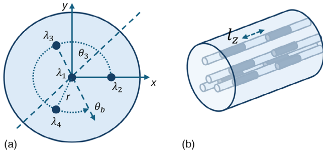
FIGURE 3 (a) Representation of a 4-core MCF. \lambda_i is the wavelength of the i^{\text{th}} core, \theta_i is the counter-clockwise angle between the x -axis and the i^{\text{th}} core, while \theta_b is the bending plane angle with respect to the x -axis. (b) Isometric view of a MCF. l_z is the distance between two consecutive FBG.
