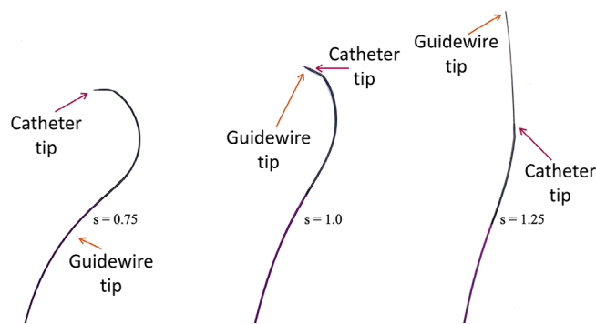
FIGURE 2 Illustration of the straightening effect of the catheter that occurs when a stiff guidewire is pushed through the catheter. As the guidewire advances, its stiffer section changes the shape of the catheter. The parameter ‘s’ on each image indicates the local curvilinear coordinate of the guidewire within the catheter.
