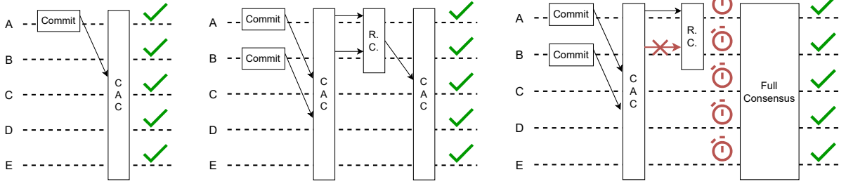
(a) In the absence of conflicts, the consensus terminates after one CAC instance.
