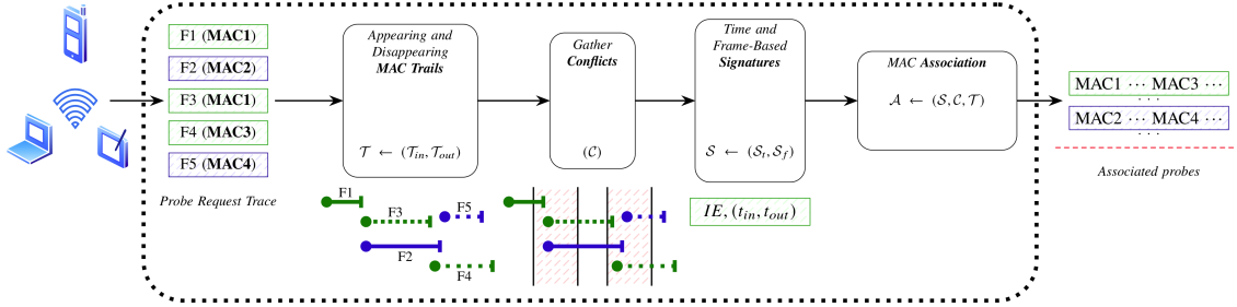
Fig. 2: Bleach framework.
