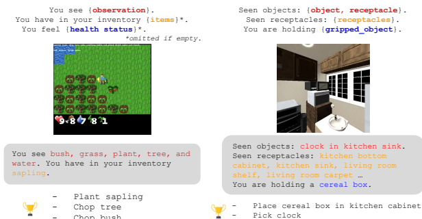
Figure 3: Sample templated captions and suggested goals.
