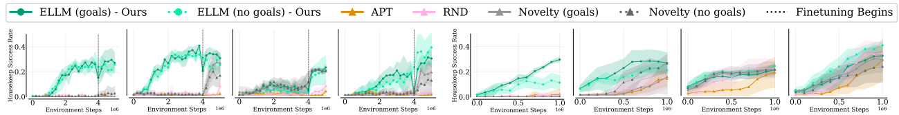
(a) Pretraining and finetuning : pretraining for 4M steps then finetuning for 1M steps on the ground truth correct arrangement. (b) Downstream evaluation : Using the frozen pretrained exploration policies only for \epsilon -greedy-style action selection for 1M steps.
