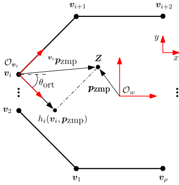
Fig. 3: The i -th DT-CBF represents the signed distance between the ZMP position and the edge connecting v_i and v_{i+1} . It is computed as the x -component of the \mathbf{p}_{\text{zmp}} expressed in the reference frame RF_{v_i} .
