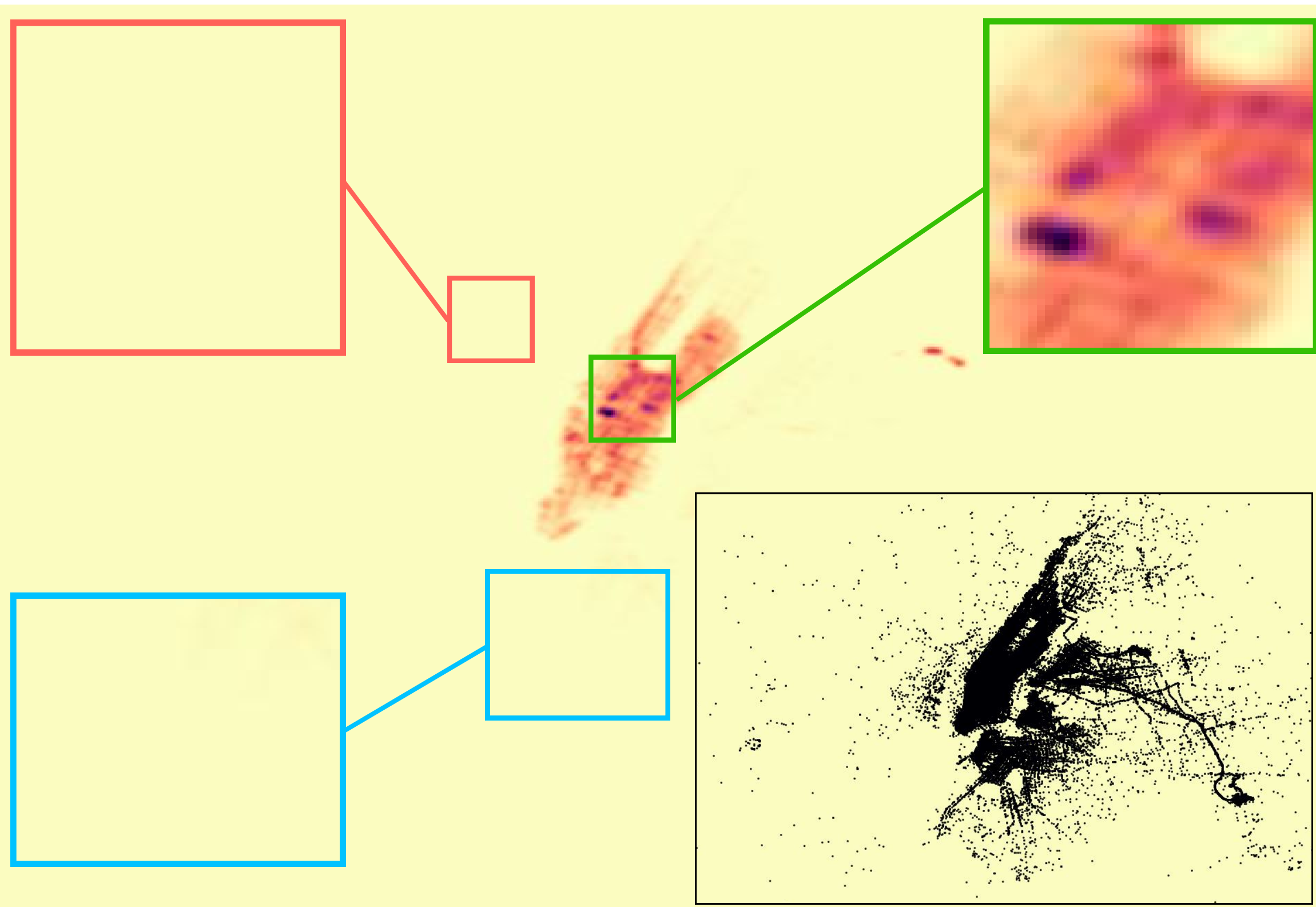
(a) Continuous density plot
