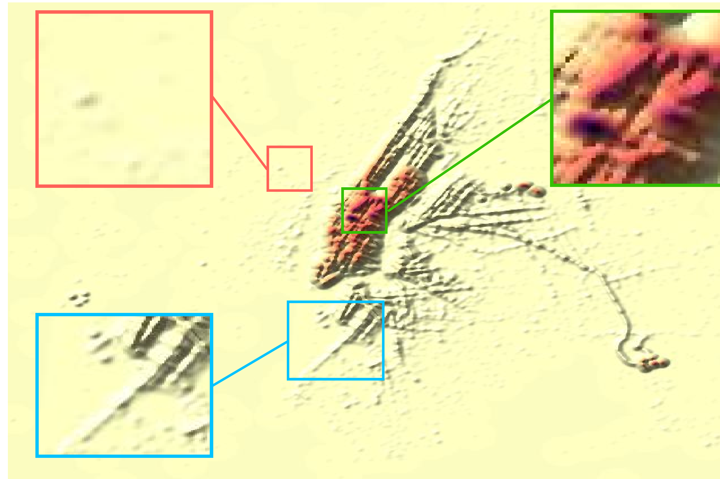
(b) Illuminated density plot
