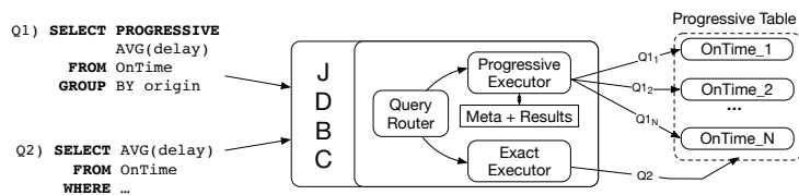
Figure 3.2: ProgressiveDB architecture
