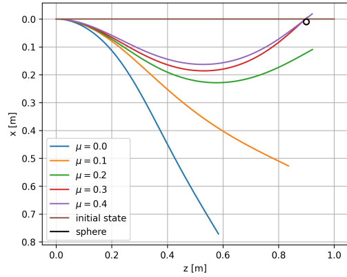
Fig. 4. Cantilever rod in frictional contact: the position of the rod is shown after 1 s of simulation for different friction coefficients, \mu . The higher the value of \mu , the longer the rod remains in contact with the sphere.
